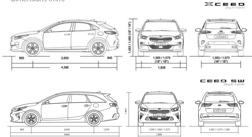
Dimensions (mm)
